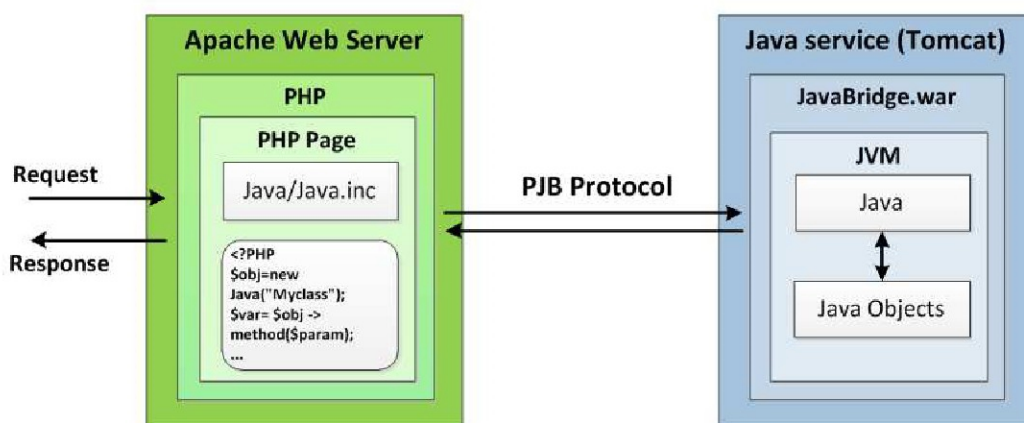
Figure 2. Desain System PHP/JavaBridge Software Scheme
